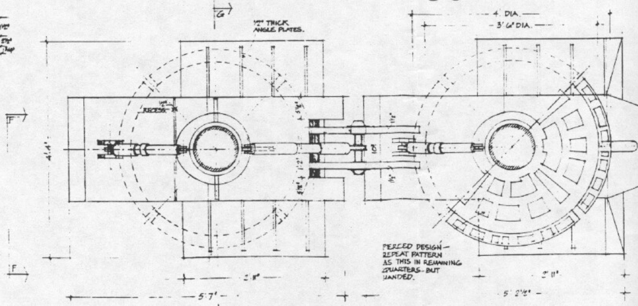
PLAN SECTION — (D D)
