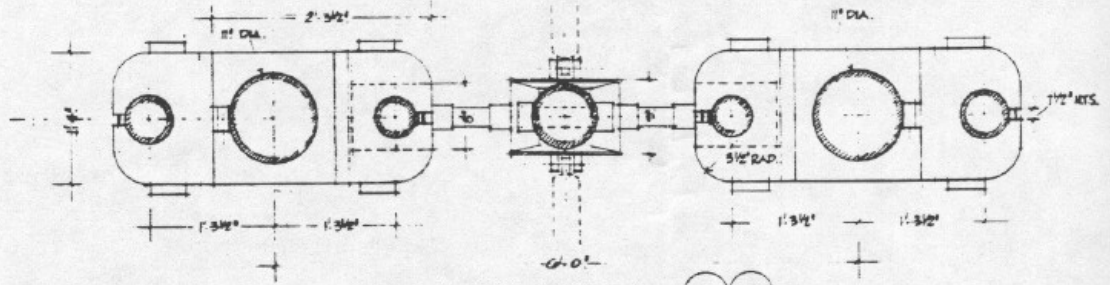
PLAN SECTION — (D D)
